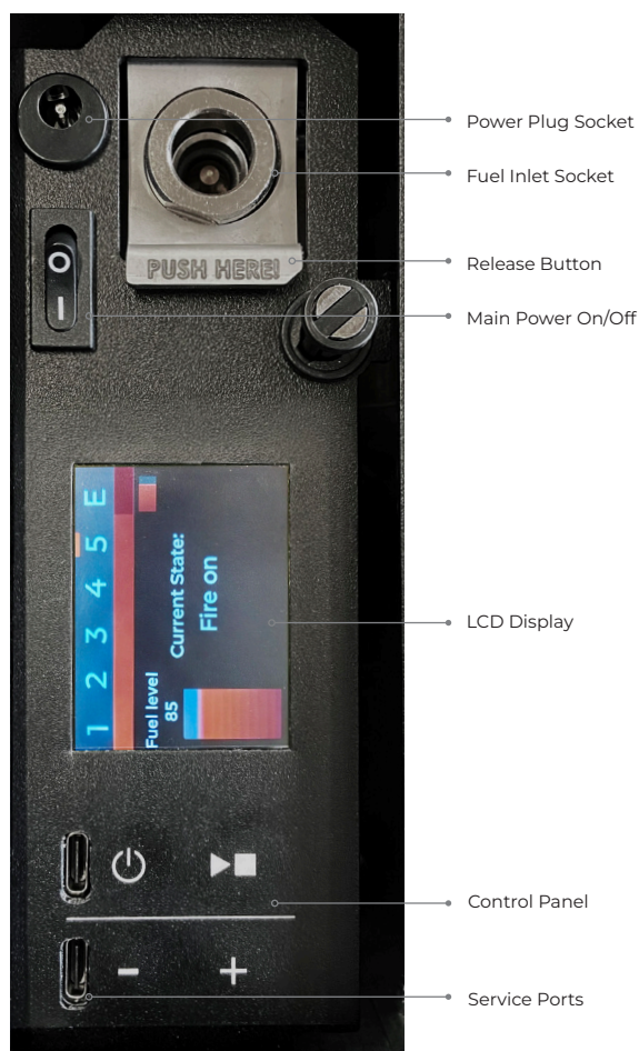
OPERATING PANEL
