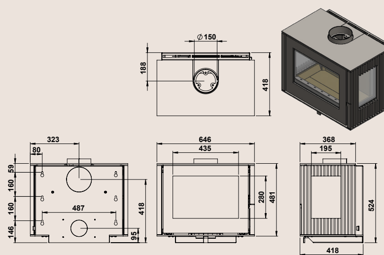
Trimline Woody loft Aero 0
